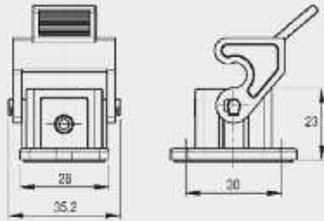
Montageausschnitt/Panel cut-out 22 x22
